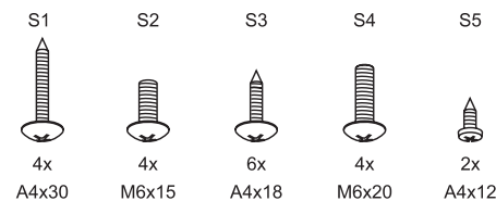
Fig. 2.1: Parts and screws for the EG2080
